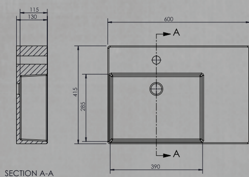
LEFT HAND BOWL BEN-5040L
